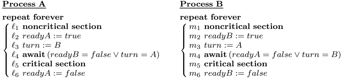
Fig. 1 Peterson’s algorithm (pseudocode)
